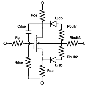
Fig. 6. MOSFET substrate network model
