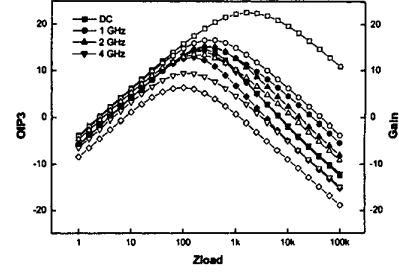
Fig. 8. Gain and OIP3 including substrate network effect
