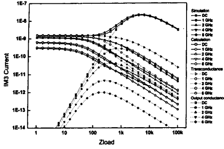
Fig. 7. The 3rd order intermodulation current with substrate network
